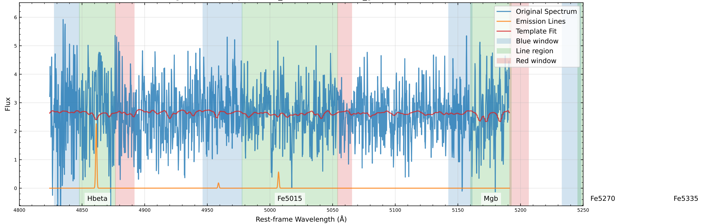
Original Data Comparison (v_star=-466.2 km/s, v_gas=-398.4 km/s)
