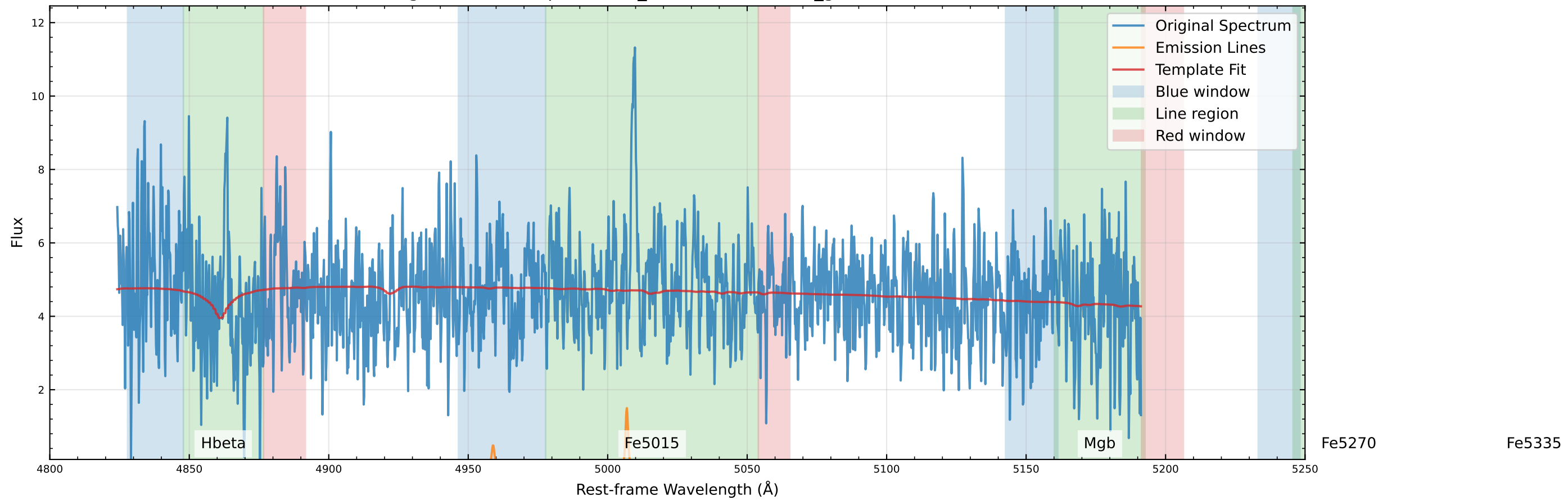
Original Data Comparison (v_star=-39.3 km/s, v_gas=-46.6 km/s)
