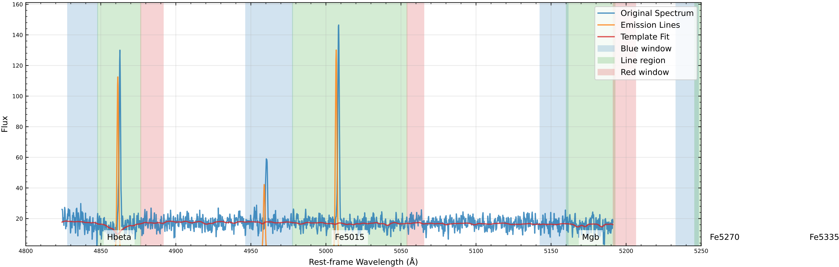
Original Data Comparison (v_star=44.8 km/s, v_gas=89.5 km/s)
