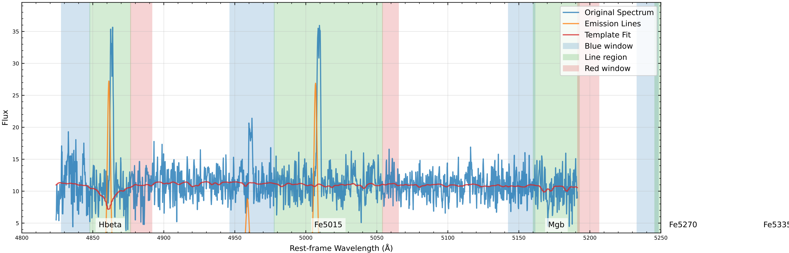
Original Data Comparison (v_star=134.2 km/s, v_gas=128.5 km/s)
