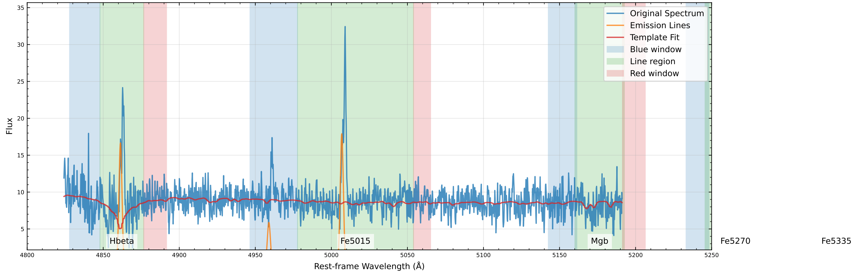
Original Data Comparison (v_star=47.8 km/s, v_gas=106.2 km/s)
