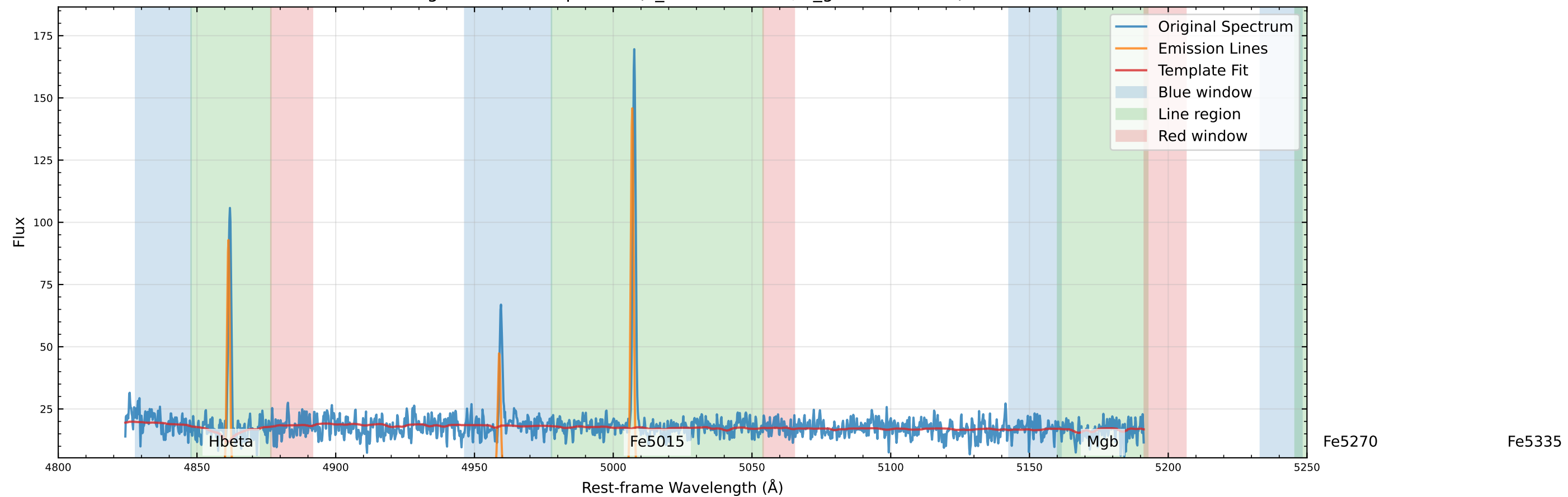
Original Data Comparison (v_star=1.2 km/s, v_gas=39.6 km/s)
