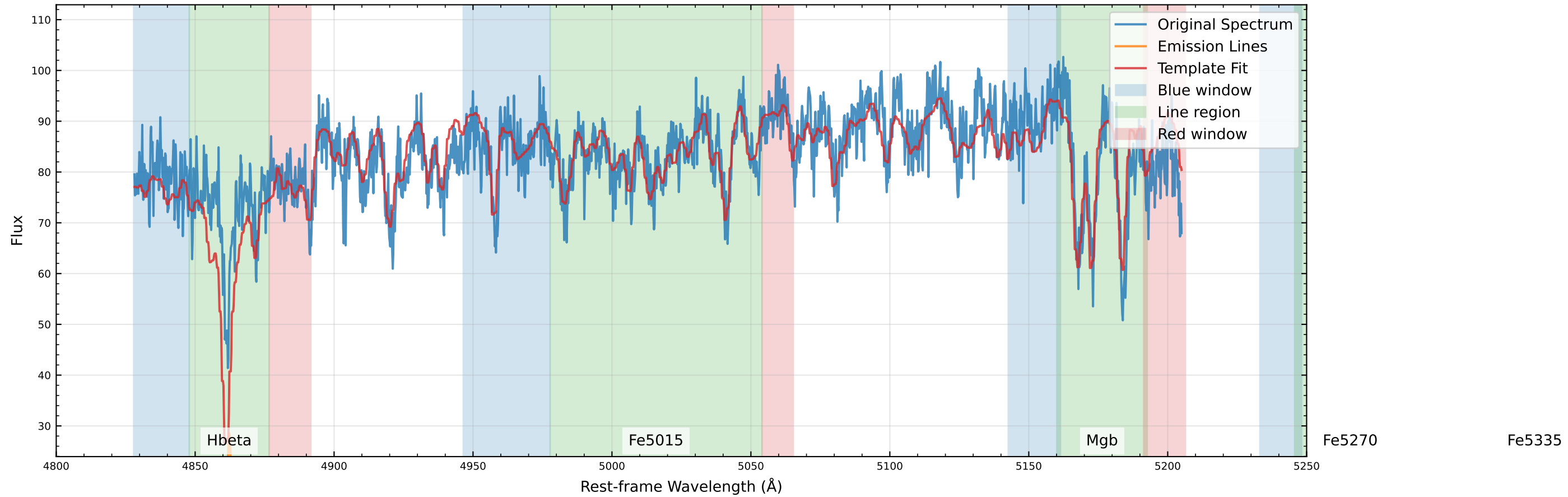
Original Data Comparison (v_star=26.2 km/s)
