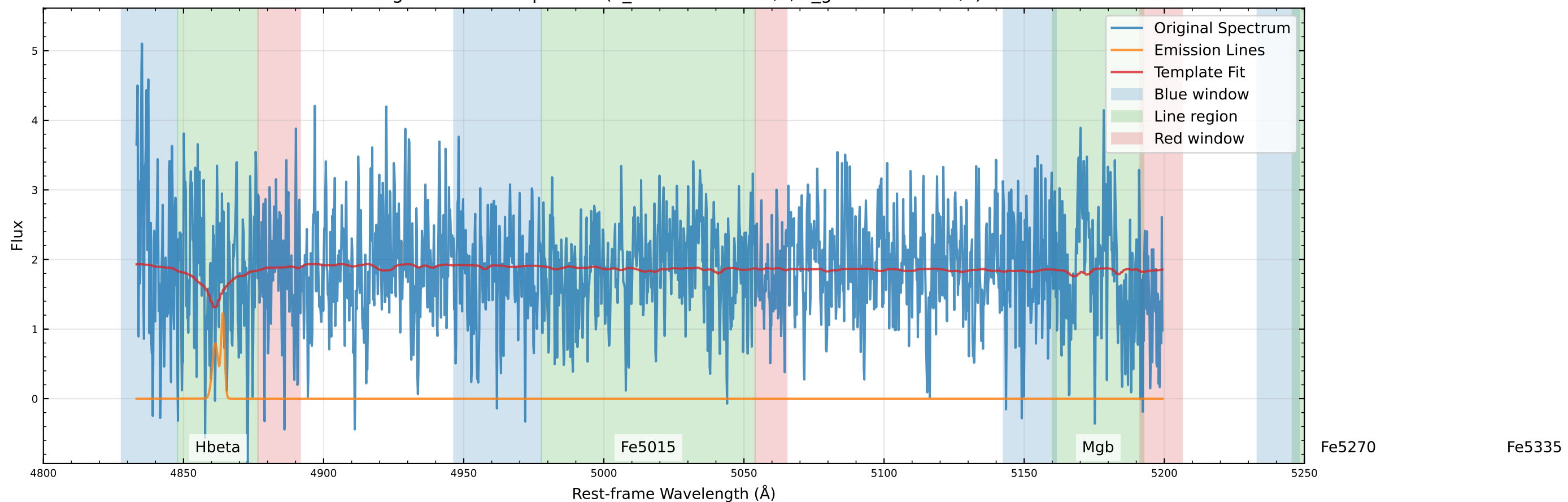
Original Data Comparison (v_star=-386.2 km/s, v_gas=-511.0 km/s)
