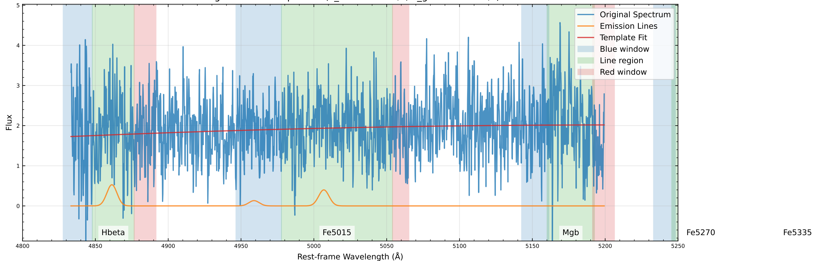
Original Data Comparison (v_star=0.0 km/s, v_gas=-74.9 km/s)
