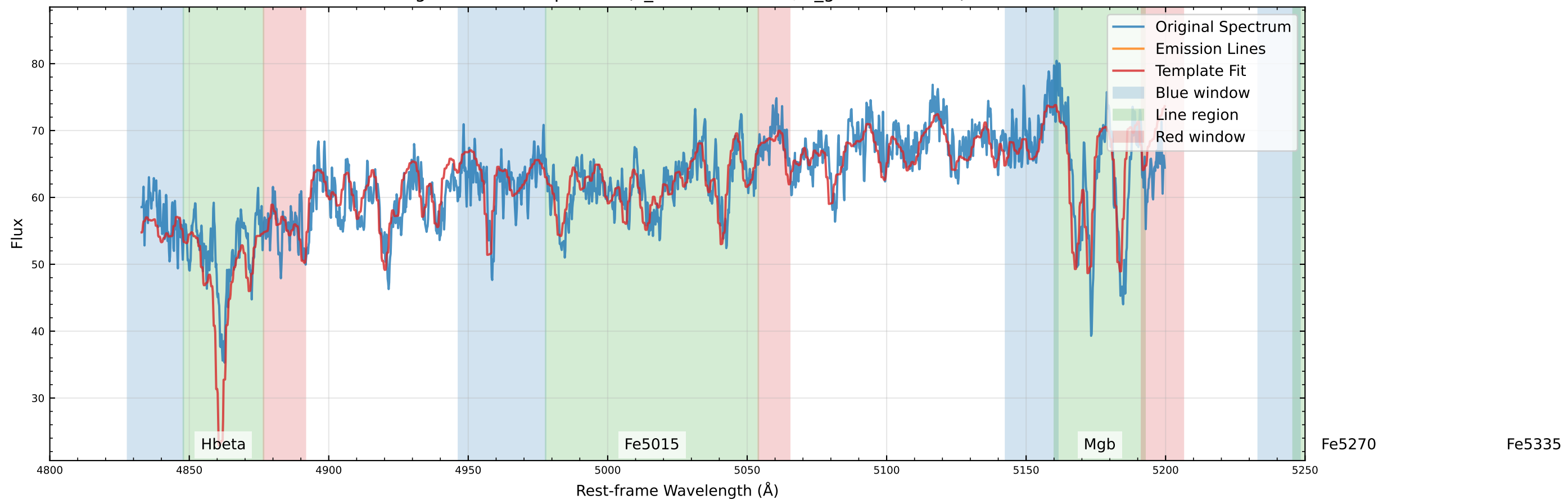
Original Data Comparison (v_star=56.5 km/s, v_gas=54.0 km/s)
