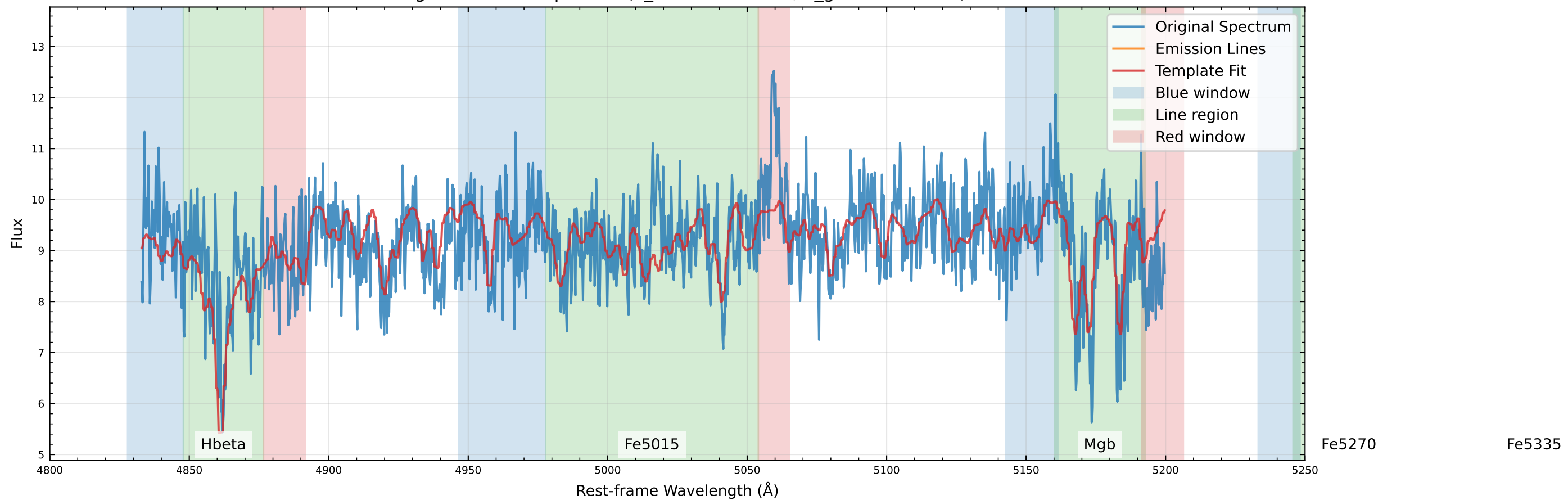
Original Data Comparison (v_star=45.9 km/s, v_gas=66.1 km/s)
