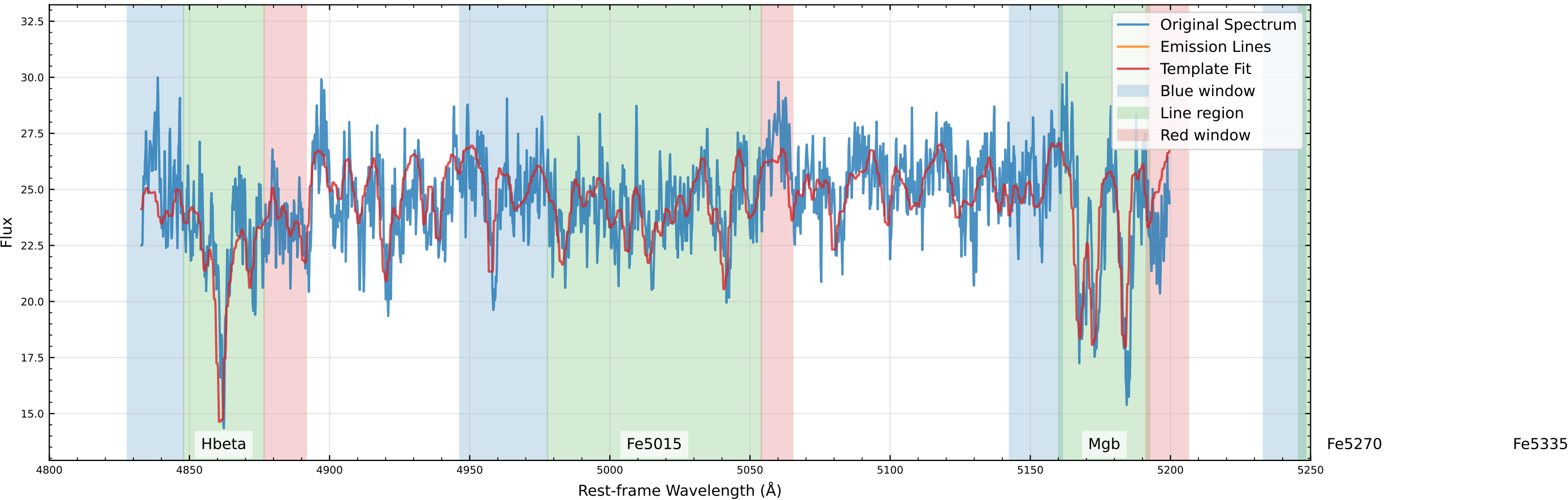
Original Data Comparison (v_star=62.7 km/s, v_gas=193.4 km/s)
