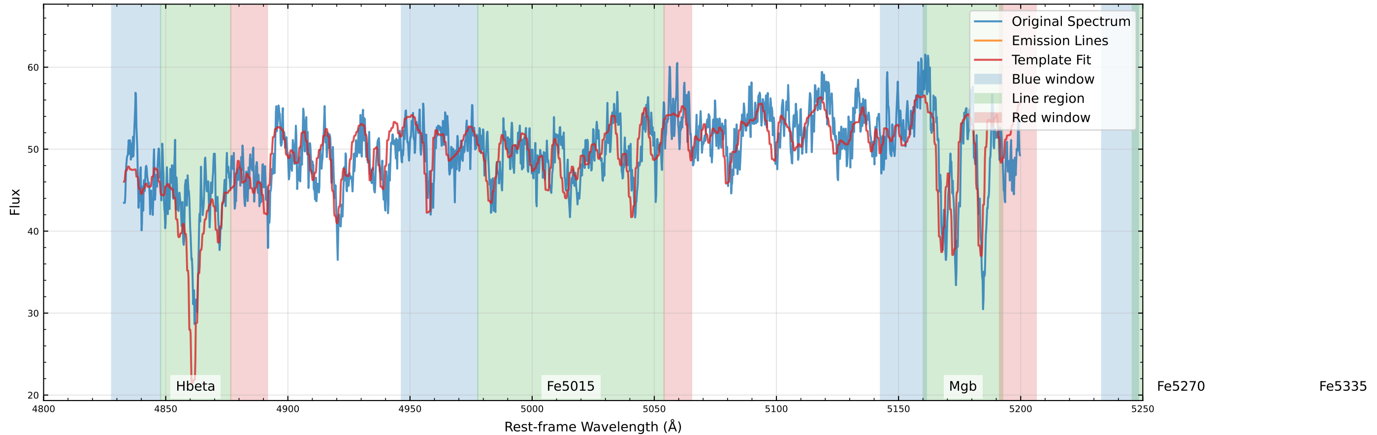
Original Data Comparison (v_star=66.6 km/s, v_gas=120.4 km/s)
