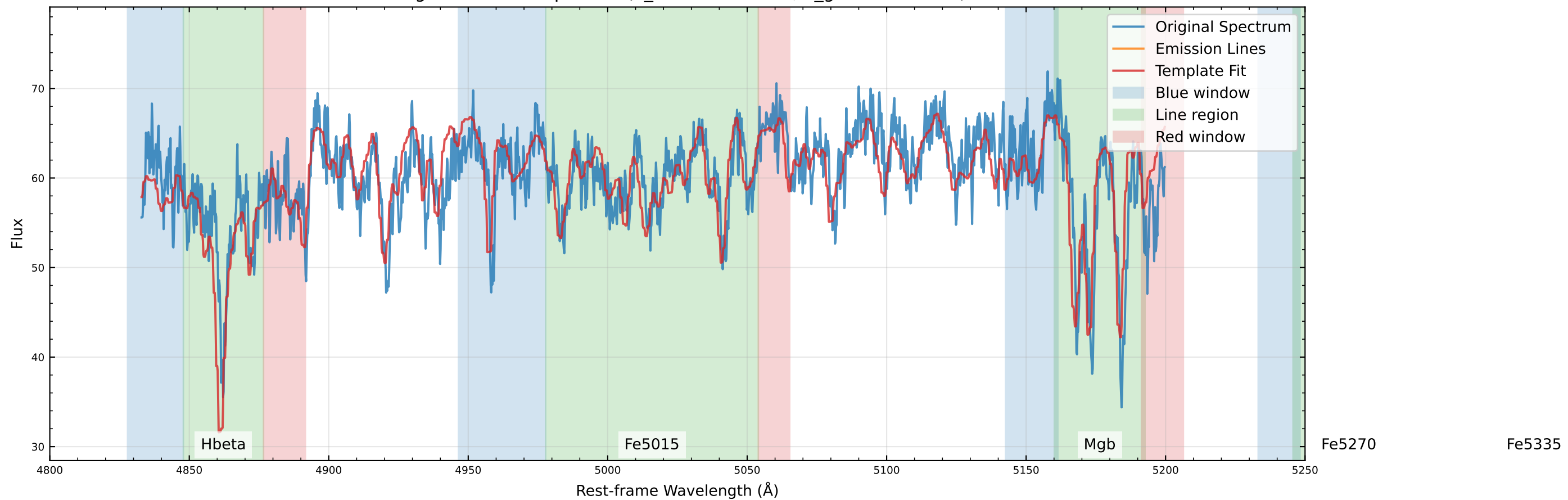
Original Data Comparison (v_star=53.5 km/s, v_gas=50.8 km/s)
