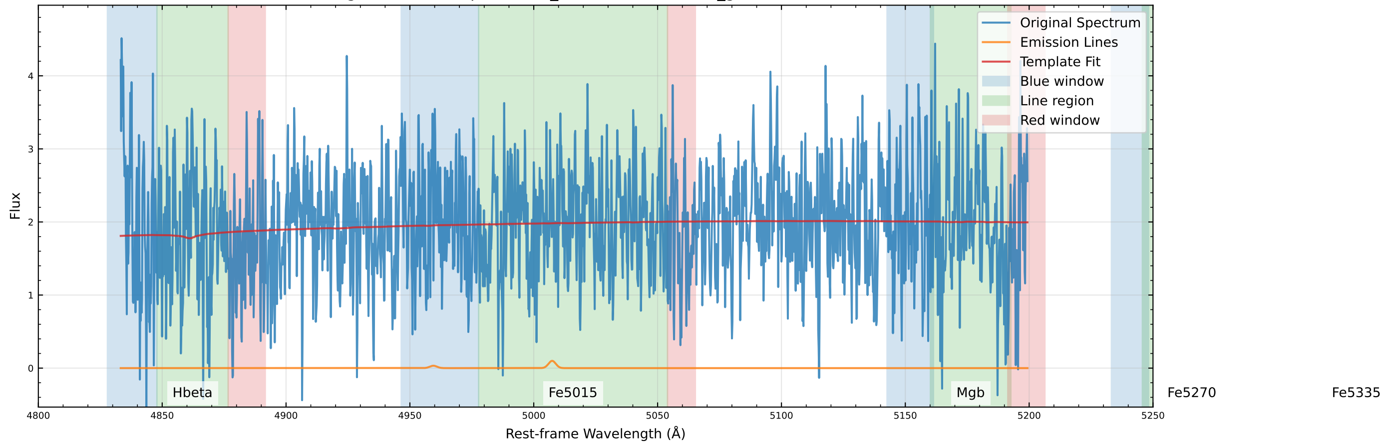
Original Data Comparison (v_star=-177.4 km/s, v_gas=-177.9 km/s)
