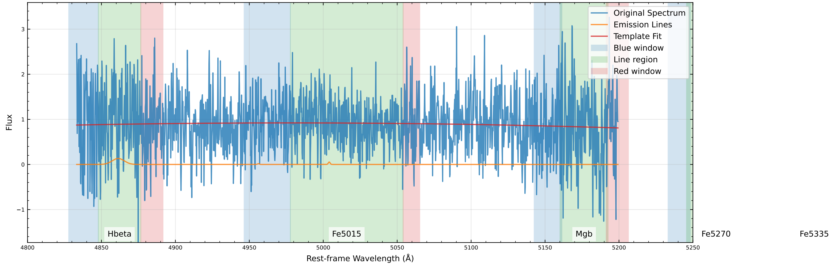
Original Data Comparison (v_star=229.8 km/s, v_gas=401.4 km/s)
