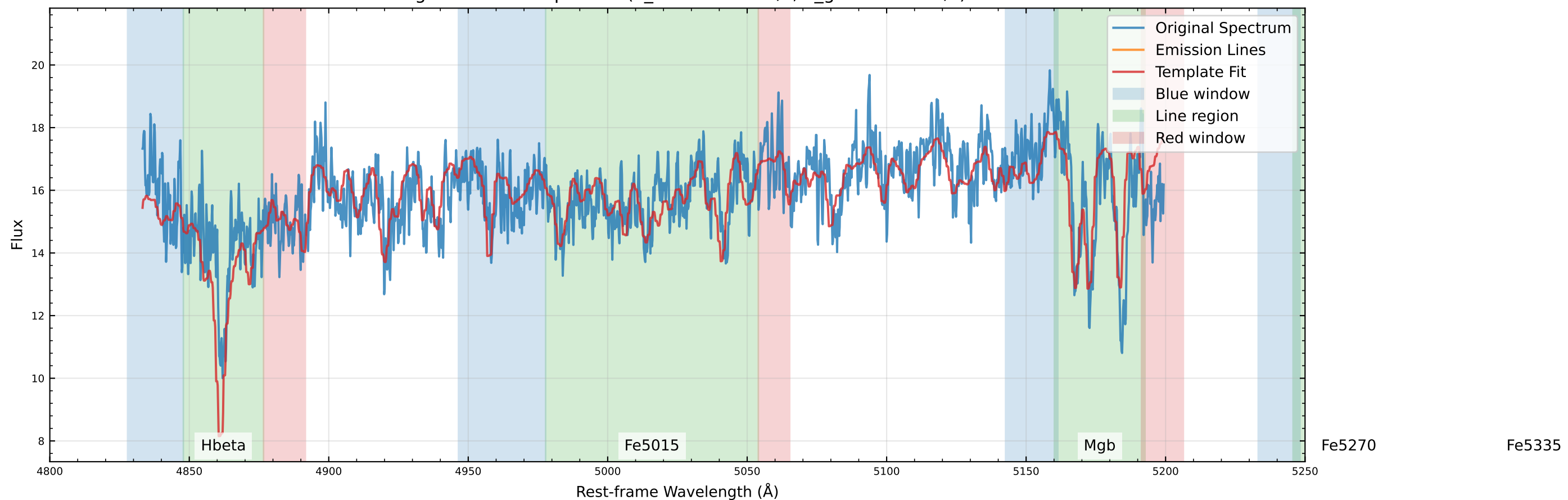
Original Data Comparison (v_star=51.9 km/s, v_gas=81.2 km/s)
