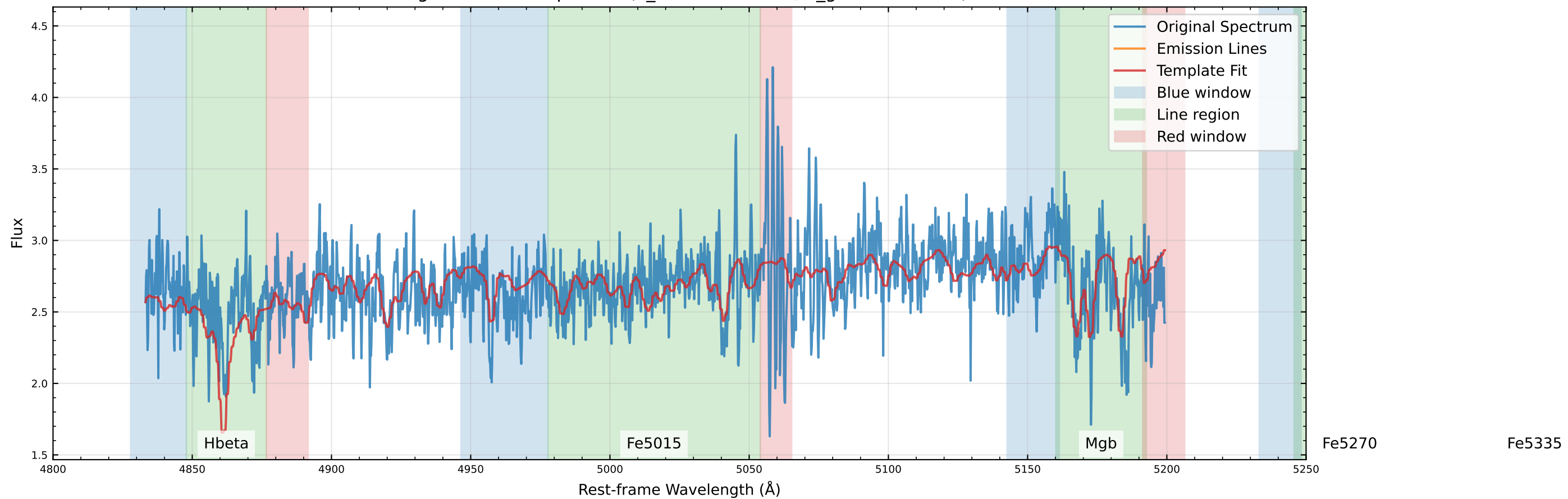
Original Data Comparison (v_star=44.8 km/s, v_gas=90.8 km/s)
