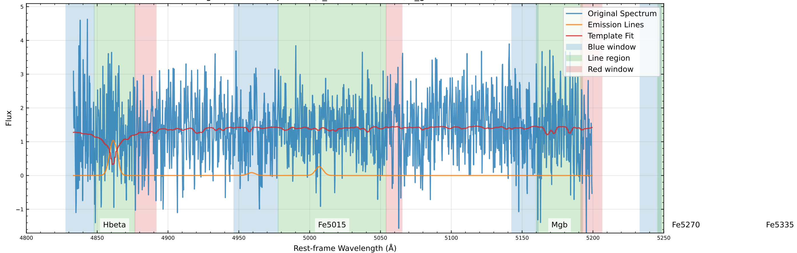
Original Data Comparison (v_star=390.6 km/s, v_gas=197.9 km/s)
