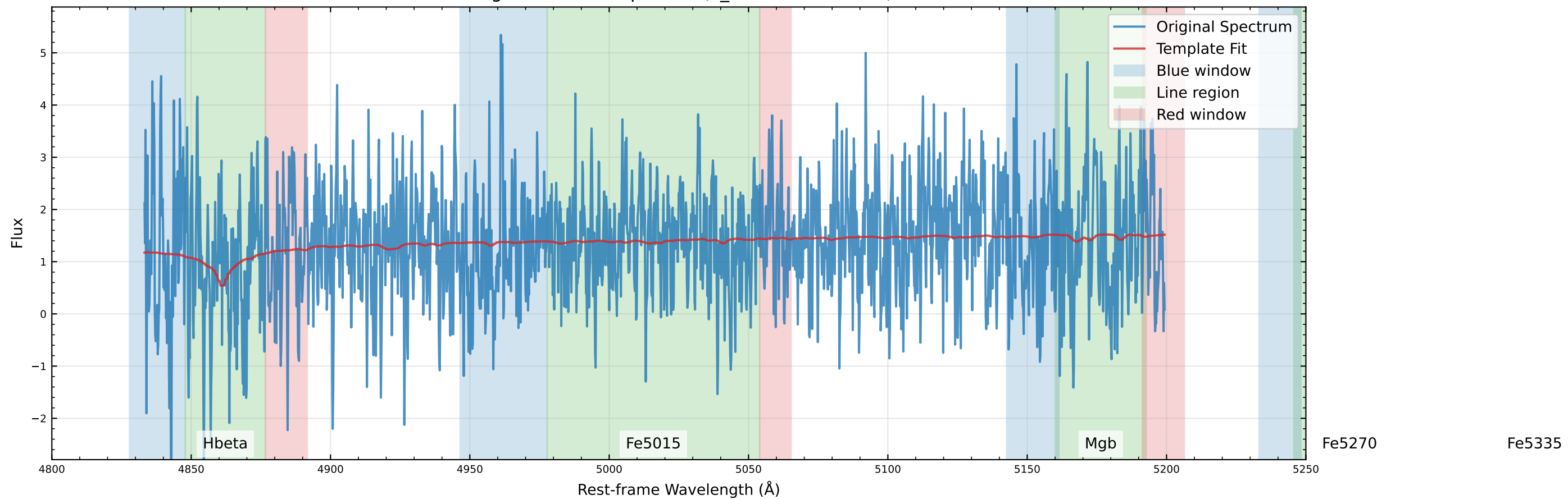
Original Data Comparison (v_star=-221.4 km/s)
