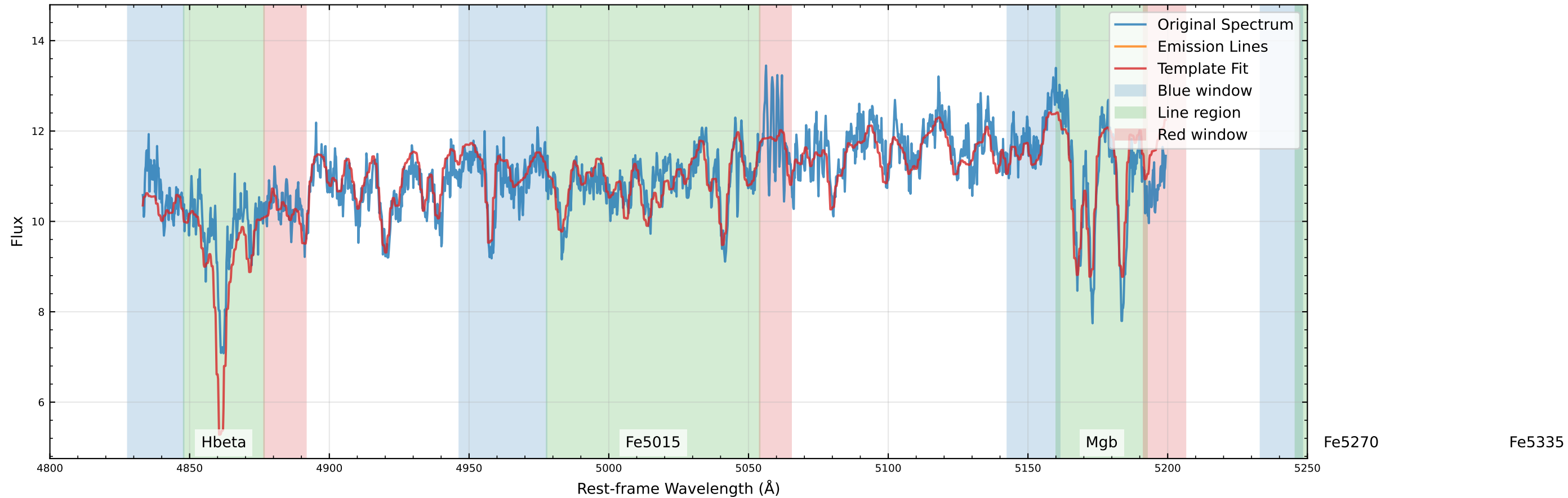
Original Data Comparison (v_star=28.5 km/s, v_gas=97.8 km/s)
