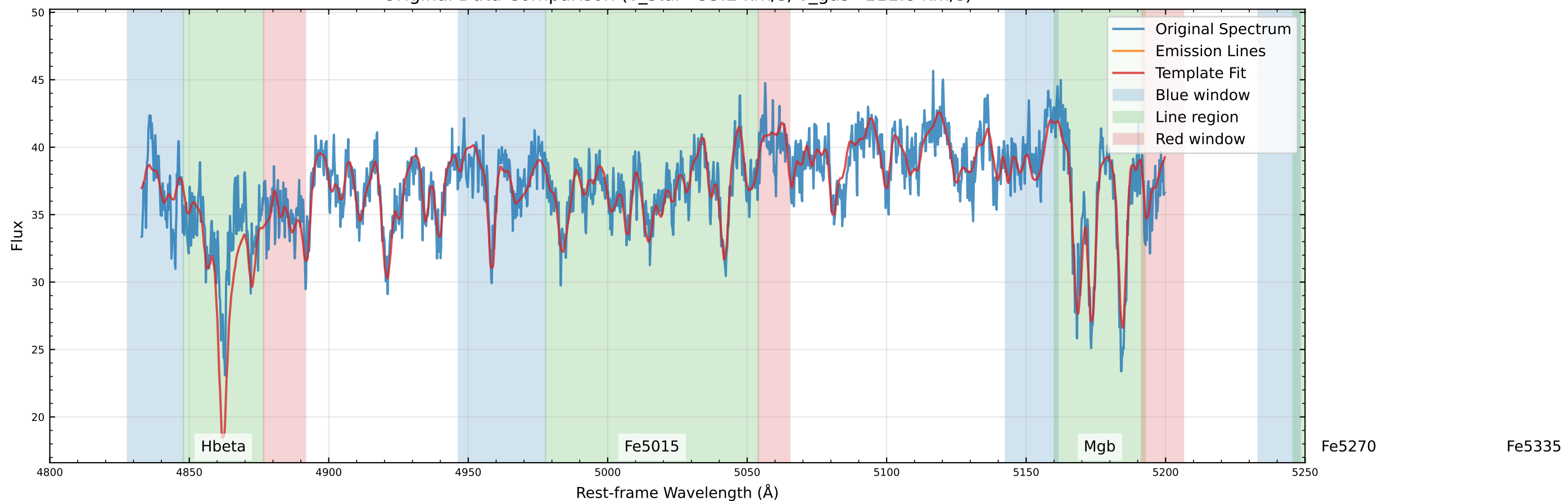
Original Data Comparison (v_star=55.2 km/s, v_gas=111.8 km/s)
