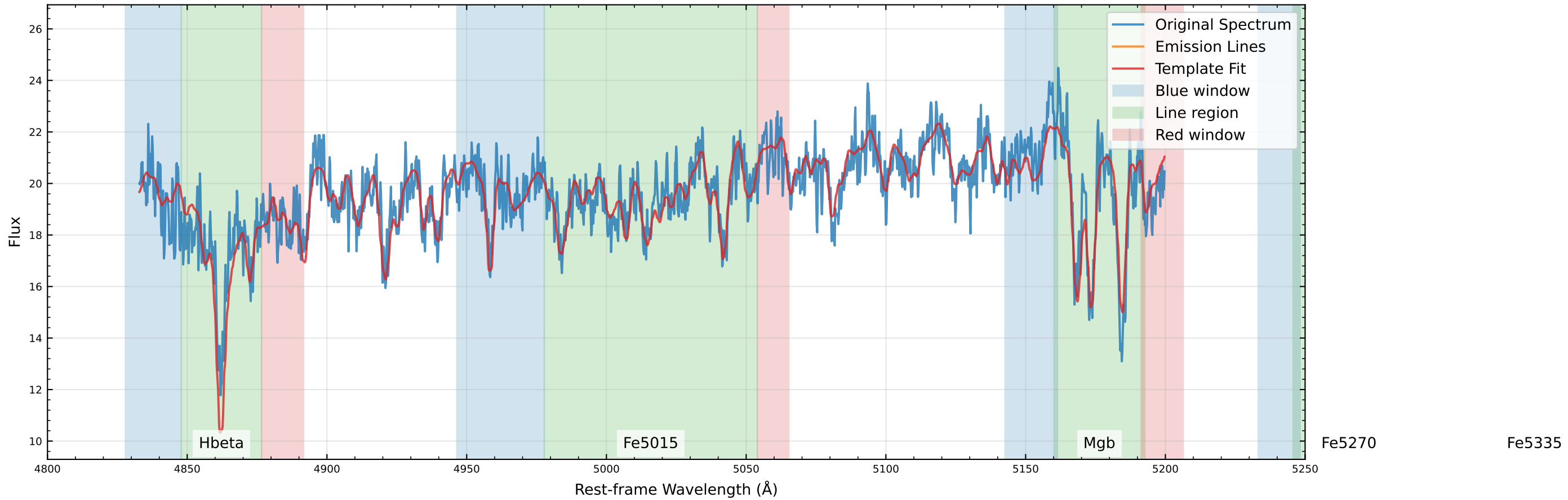
Original Data Comparison (v_star=51.8 km/s, v_gas=73.6 km/s)
