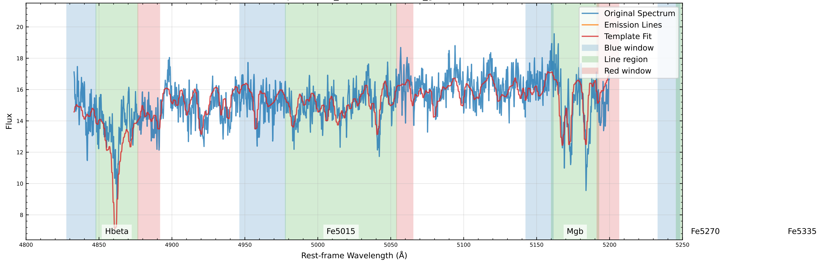
Original Data Comparison (v_star=61.9 km/s, v_gas=158.0 km/s)
