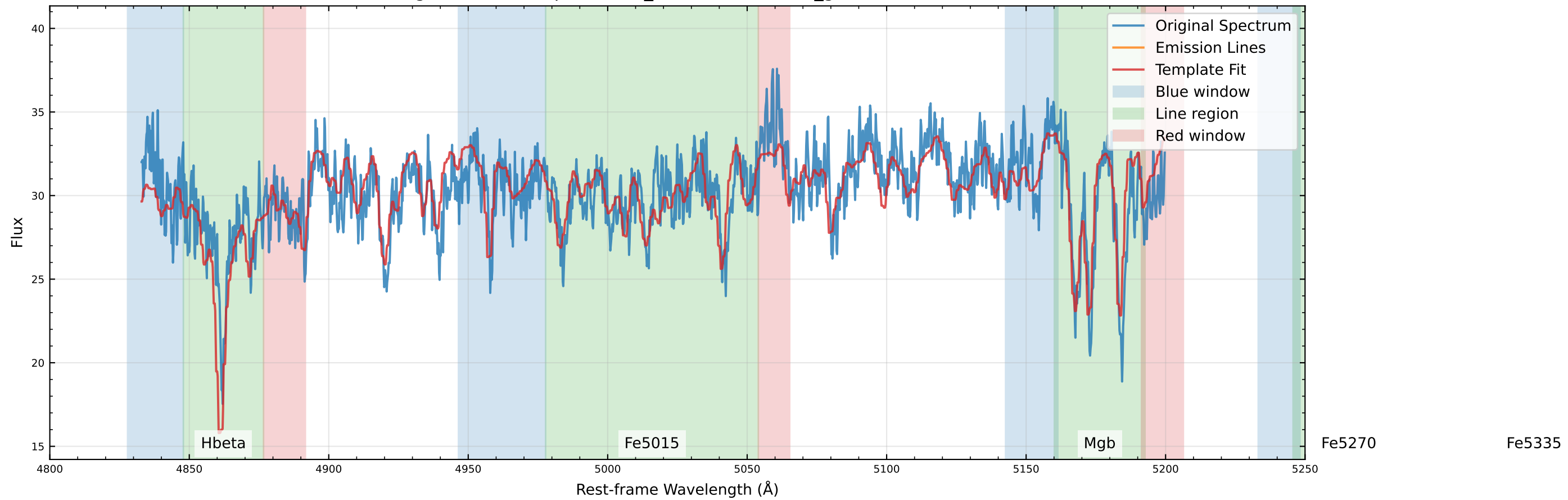
Original Data Comparison (v_star=41.1 km/s, v_gas=47.2 km/s)
