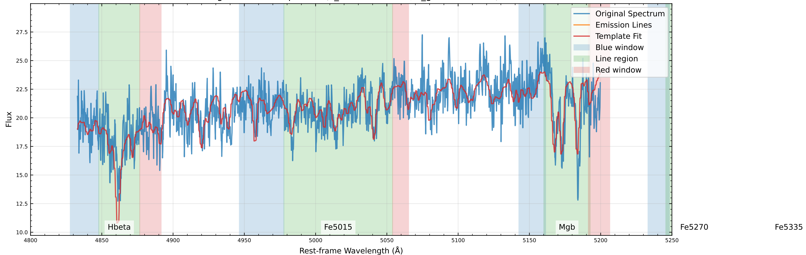
Original Data Comparison (v_star=43.4 km/s, v_gas=55.6 km/s)
