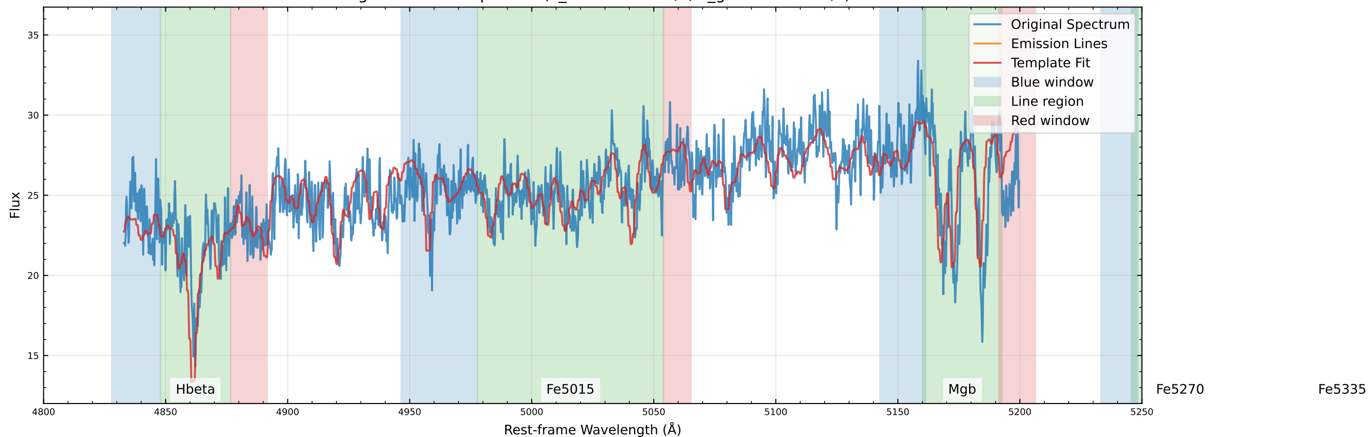
Original Data Comparison ( v_{\text{star}}=70.0 km/s, v_{\text{gas}}=106.9 km/s)
