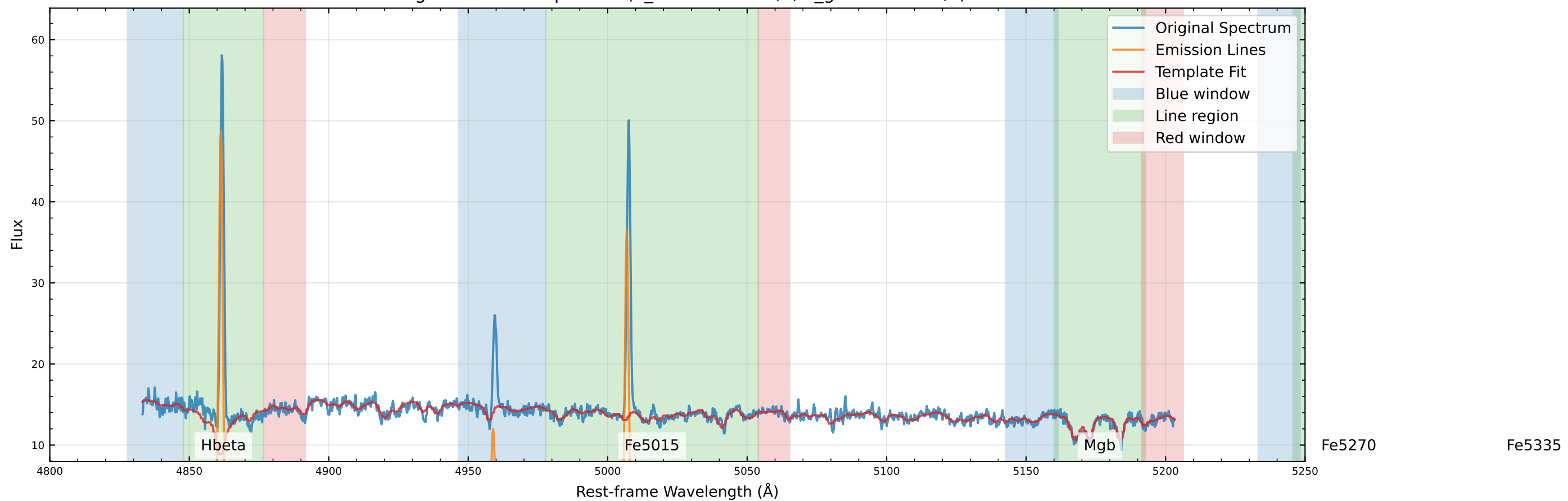
Original Data Comparison (v_star=10.4 km/s, v_gas=32.4 km/s)
