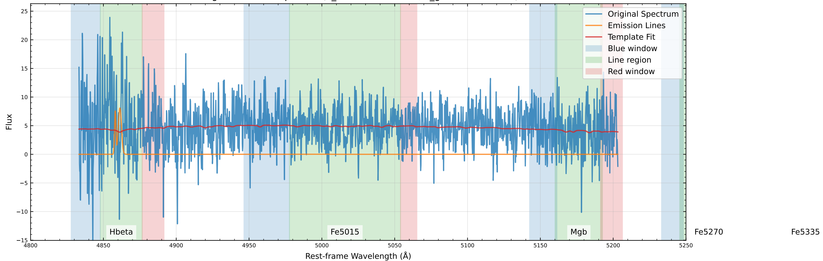
Original Data Comparison (v_star=-377.7 km/s, v_gas=-433.5 km/s)
