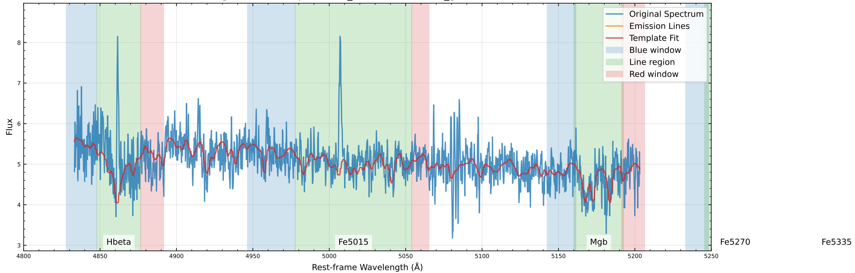
Original Data Comparison (v_star=-39.1 km/s, v_gas=20.6 km/s)
