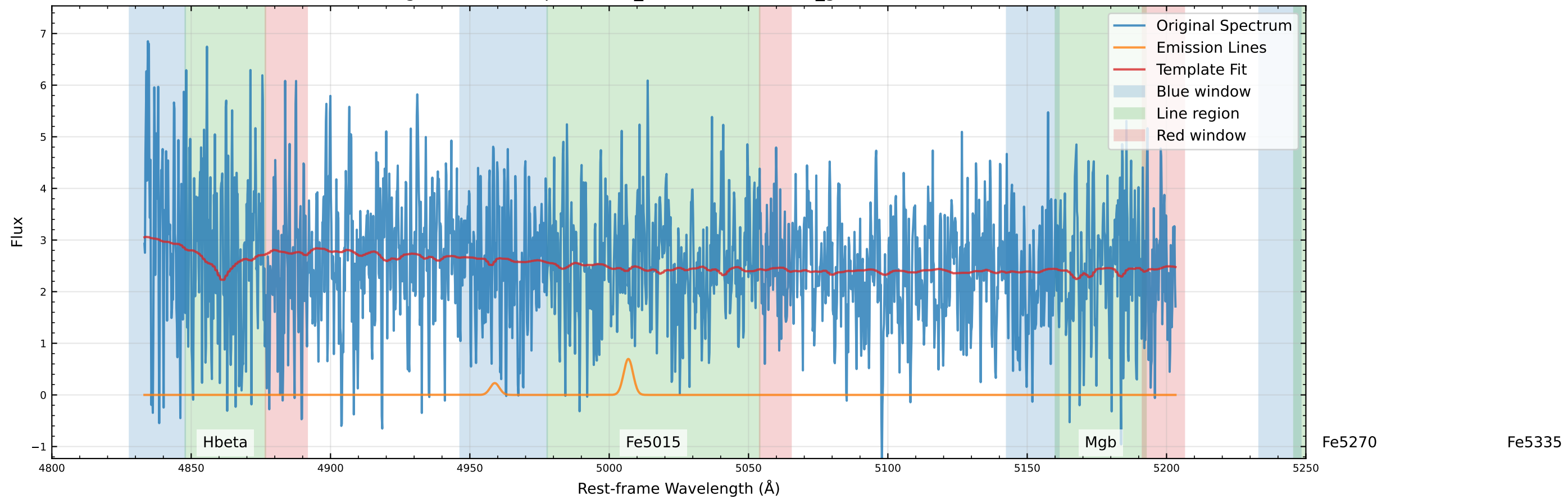
Original Data Comparison (v_star=313.9 km/s, v_gas=313.9 km/s)
