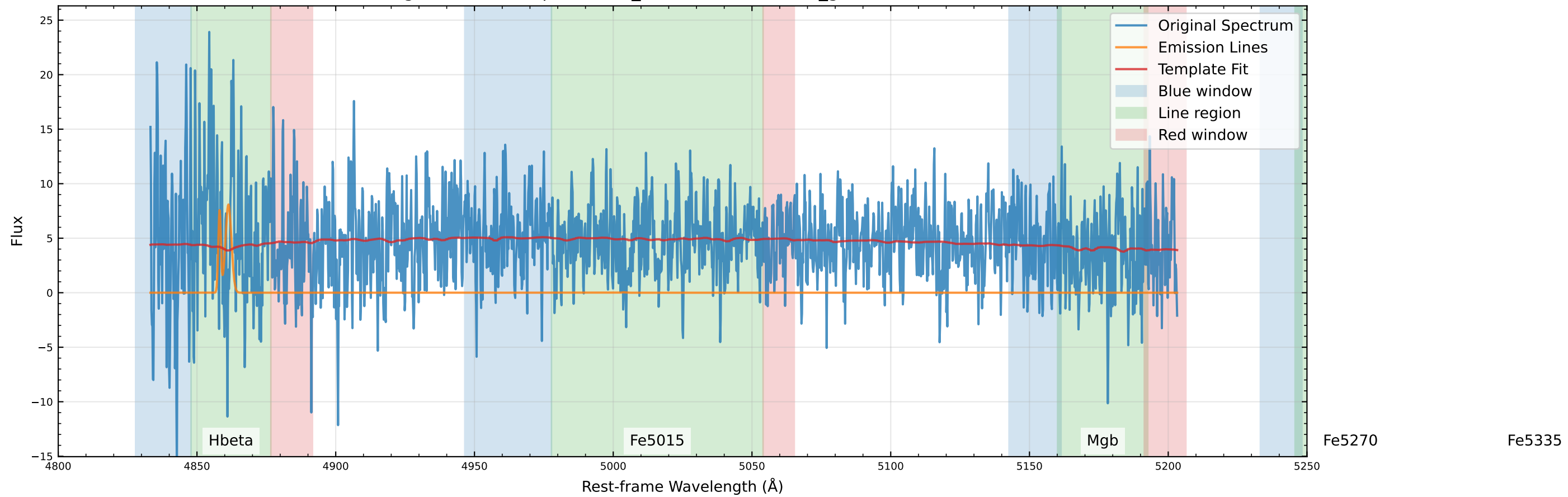
Original Data Comparison ( v_{\text{star}}=-377.7 km/s, v_{\text{gas}}=-433.5 km/s)
