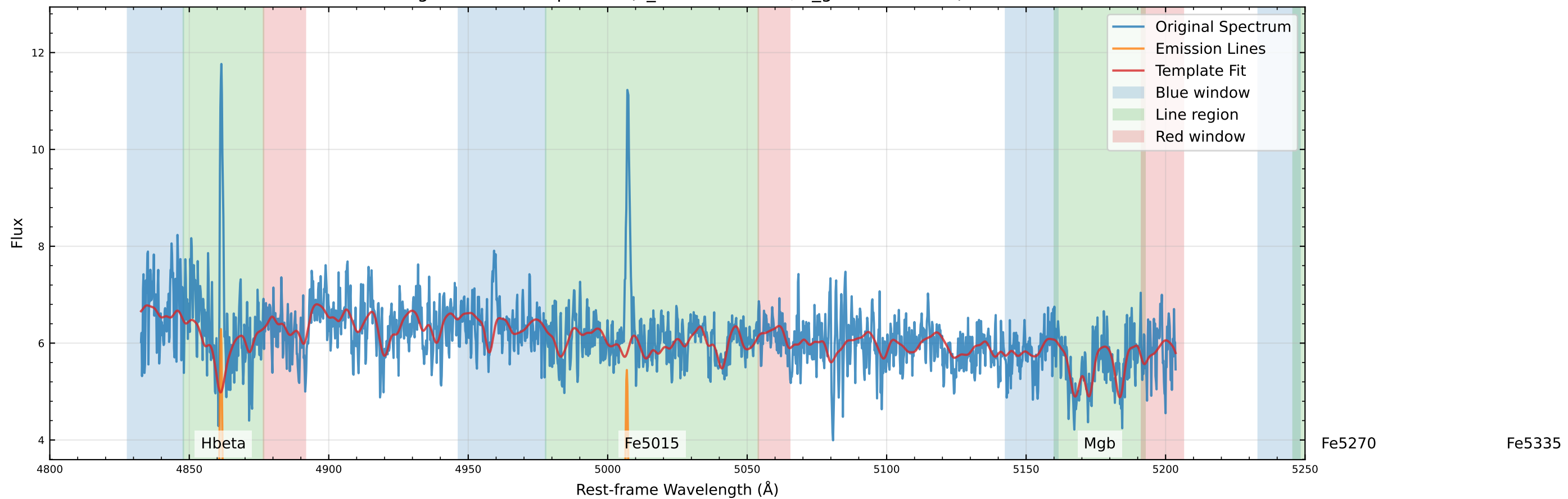
Original Data Comparison (v_star=-1.3 km/s, v_gas=17.4 km/s)
