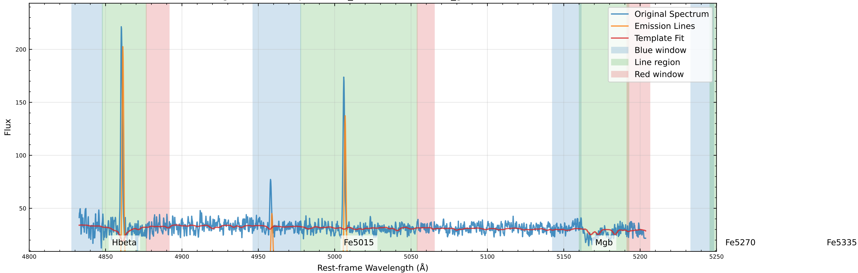
Original Data Comparison (v_star=-124.4 km/s, v_gas=-53.9 km/s)
