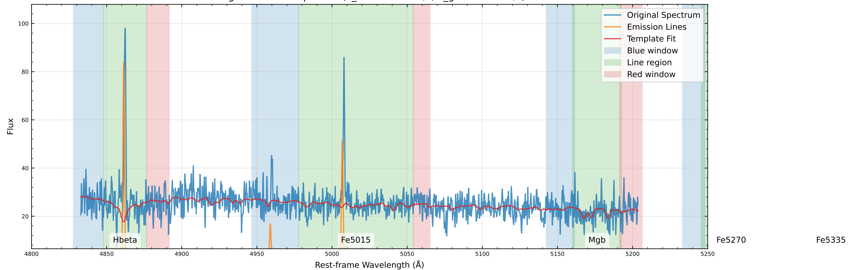
Original Data Comparison (v_star=33.6 km/s, v_gas=54.6 km/s)
