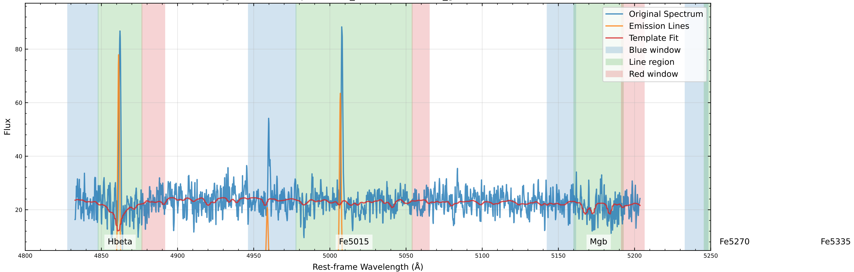
Original Data Comparison (v_star=36.0 km/s, v_gas=57.6 km/s)
