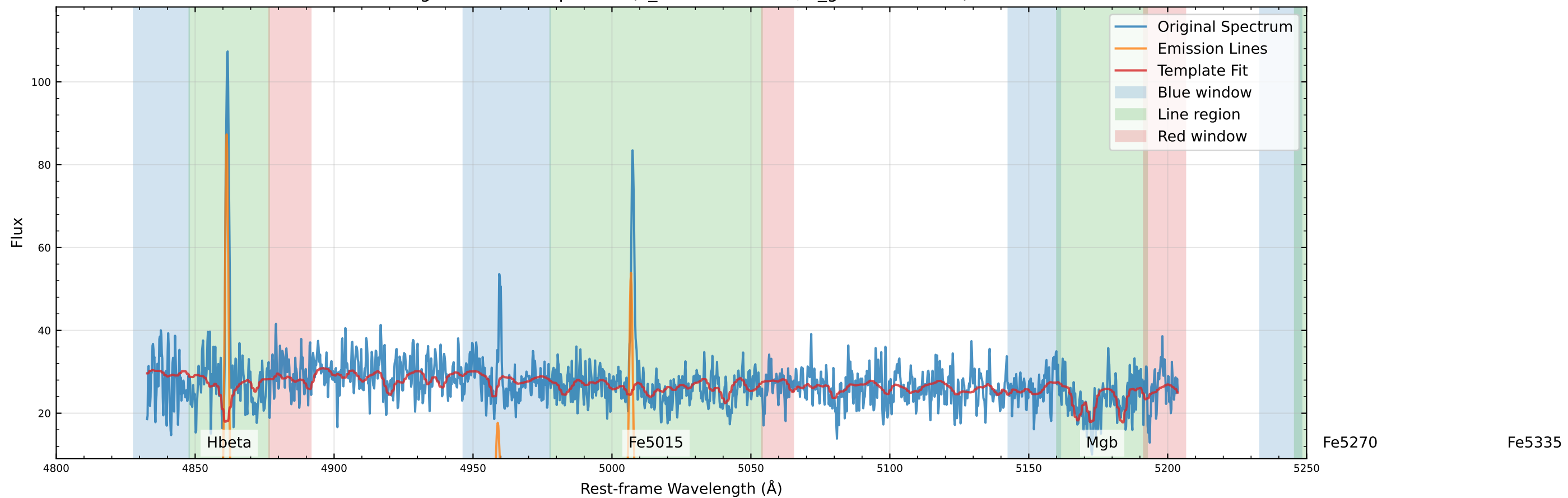
Original Data Comparison (v_star=14.7 km/s, v_gas=23.5 km/s)
