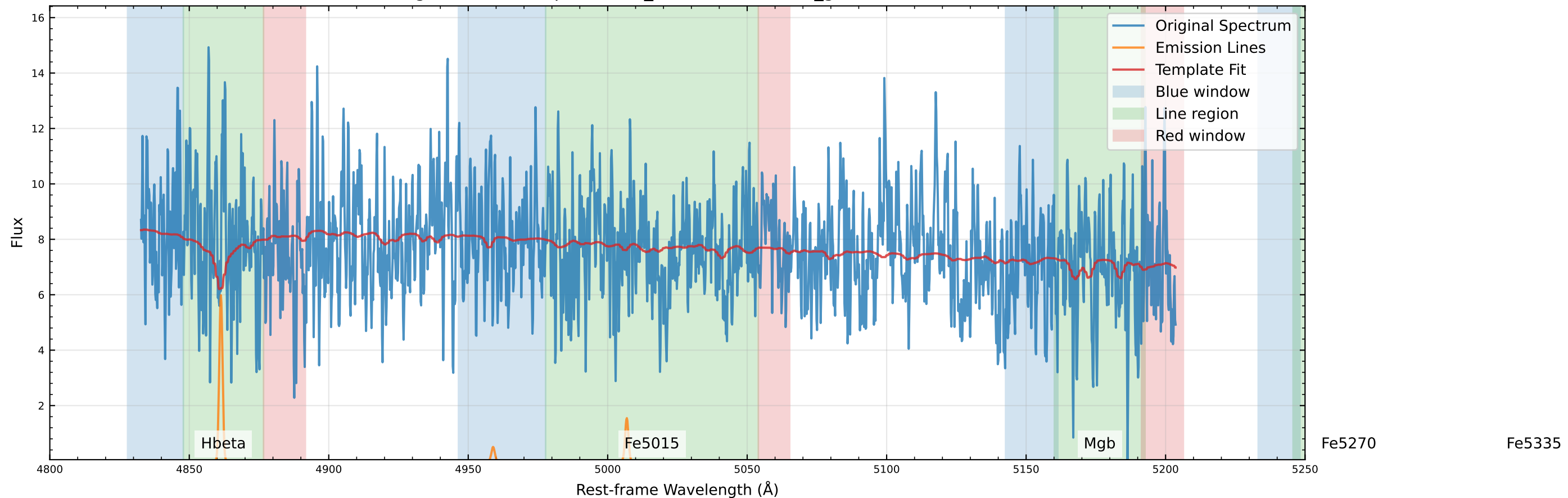
Original Data Comparison (v_star=51.8 km/s, v_gas=66.1 km/s)
