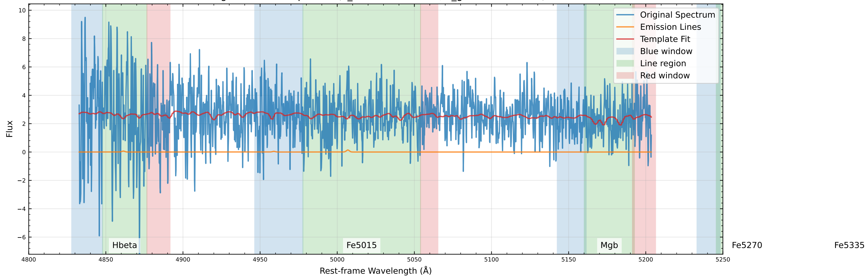
Original Data Comparison (v_star=-145.5 km/s, v_gas=-141.6 km/s)
