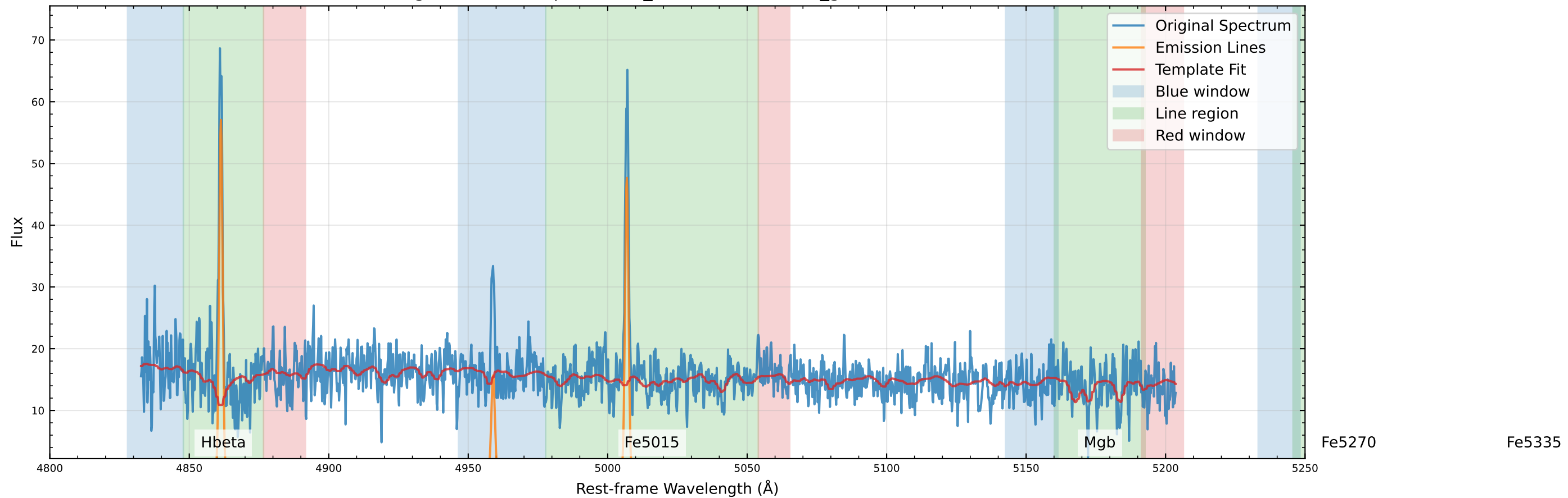
Original Data Comparison (v_star=-33.9 km/s, v_gas=-4.0 km/s)
