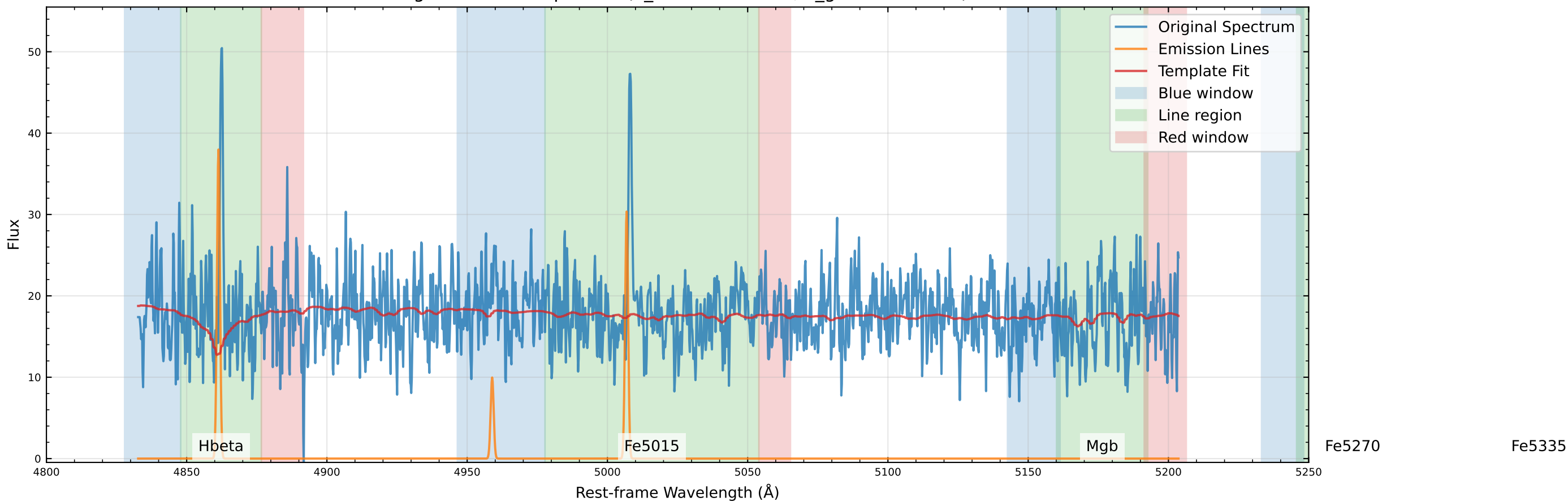
Original Data Comparison (v_star=71.1 km/s, v_gas=69.9 km/s)
