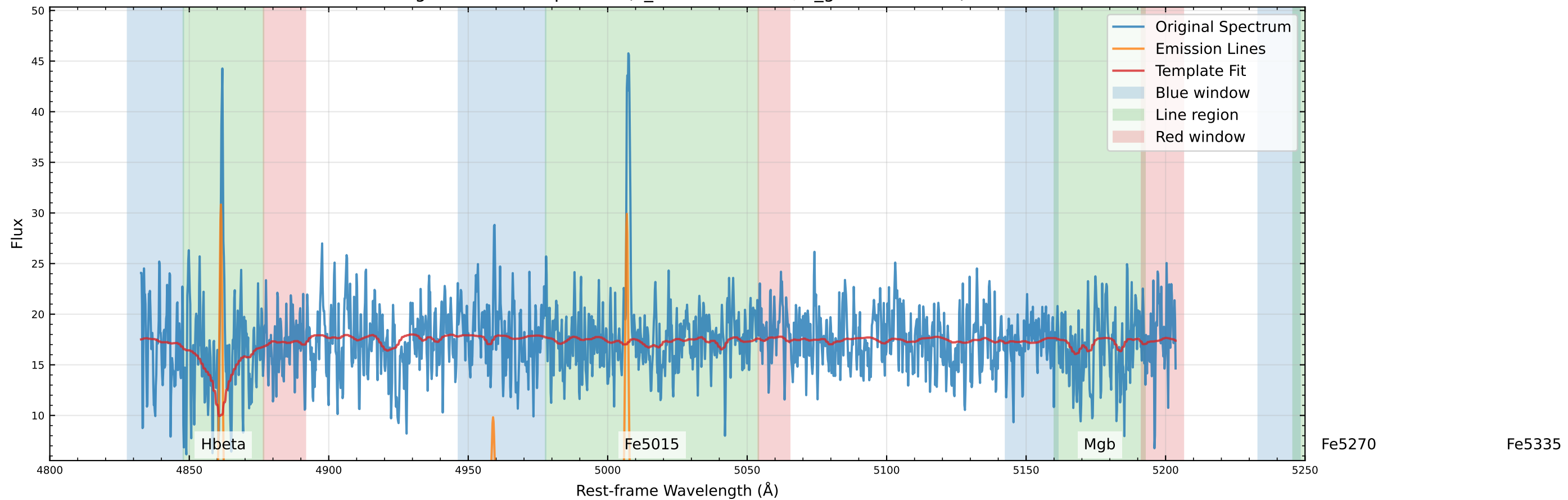
Original Data Comparison (v_star=37.9 km/s, v_gas=30.3 km/s)
