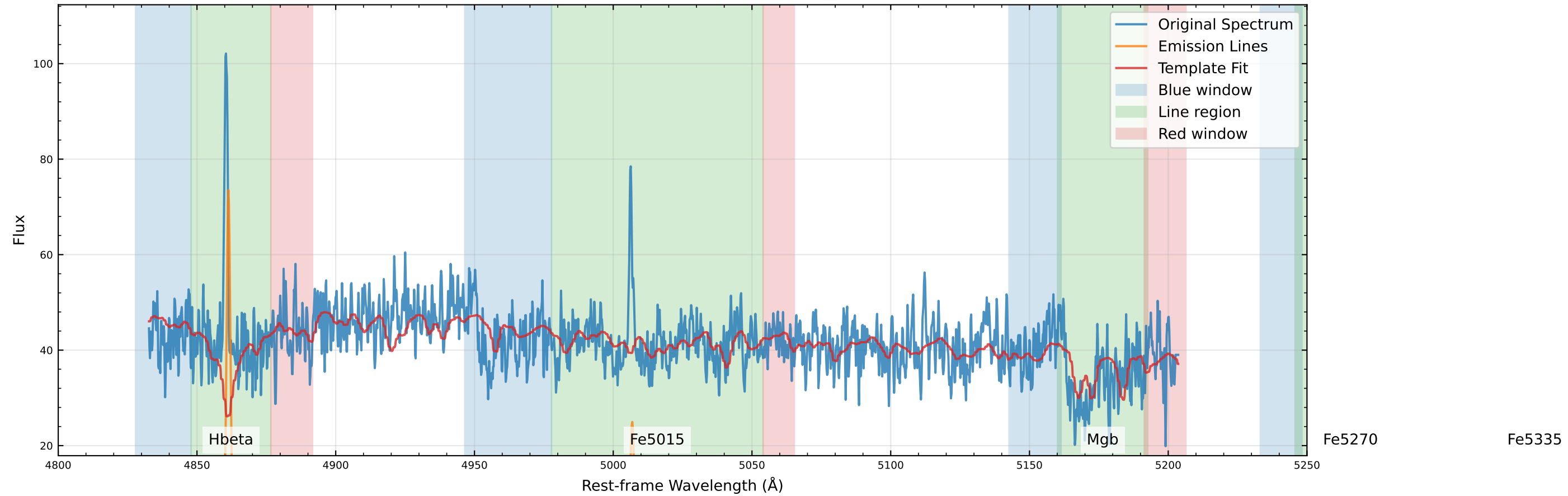
Original Data Comparison (v_star=-117.1 km/s, v_gas=-51.6 km/s)
