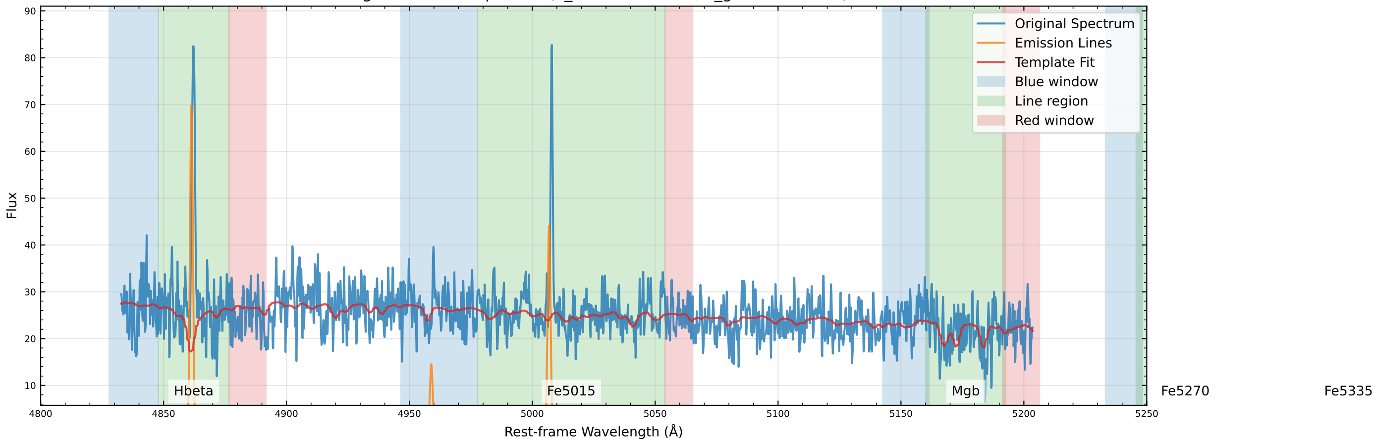
Original Data Comparison (v_star=29.4 km/s, v_gas=53.9 km/s)
