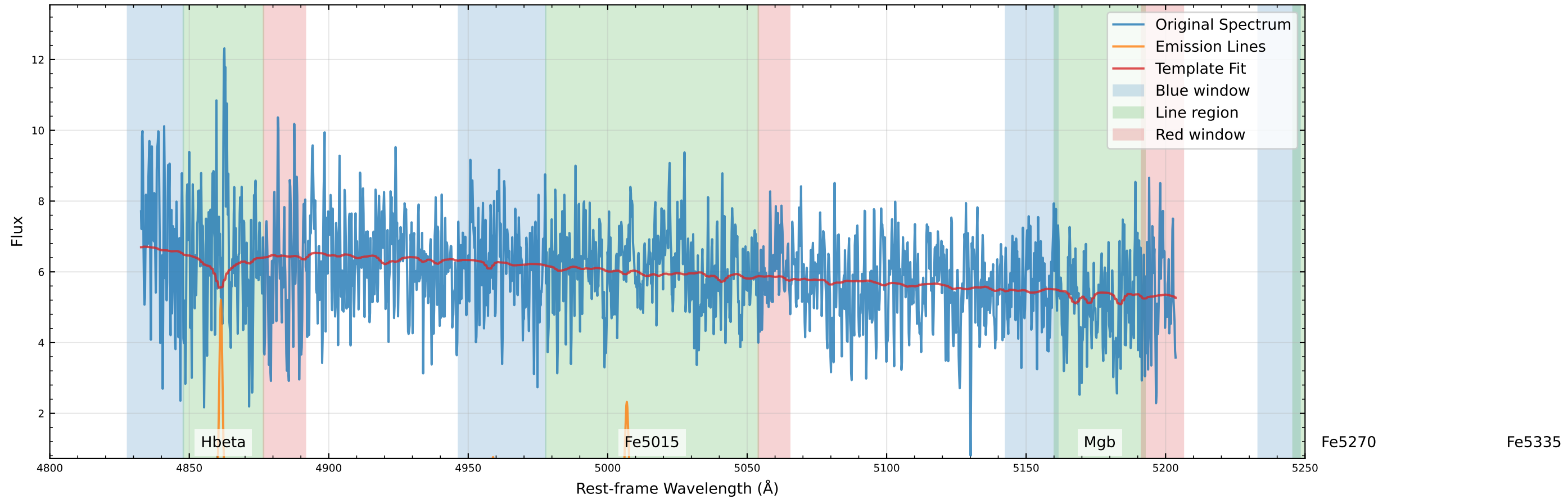
Original Data Comparison (v_star=116.6 km/s, v_gas=93.1 km/s)
