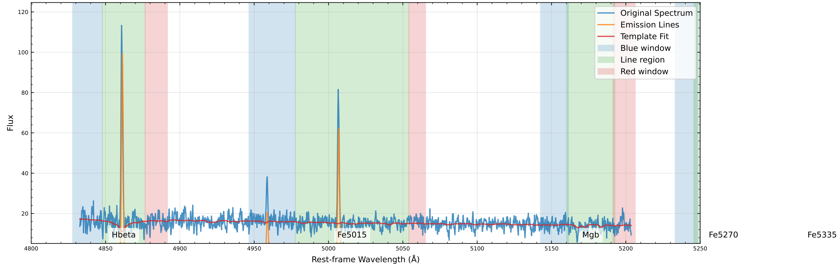
Original Data Comparison (v_star=-27.8 km/s, v_gas=-19.2 km/s)
