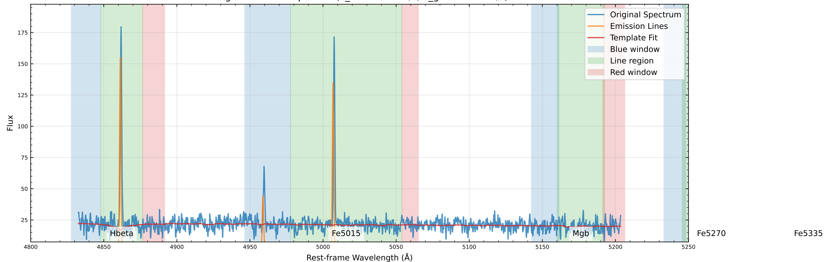
Original Data Comparison (v_star=8.5 km/s, v_gas=36.5 km/s)
