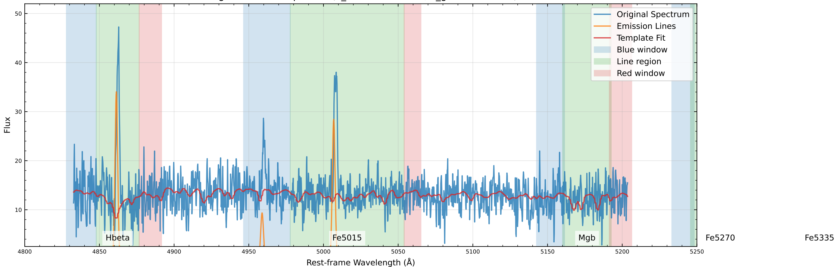
Original Data Comparison (v_star=-23.4 km/s, v_gas=73.4 km/s)
