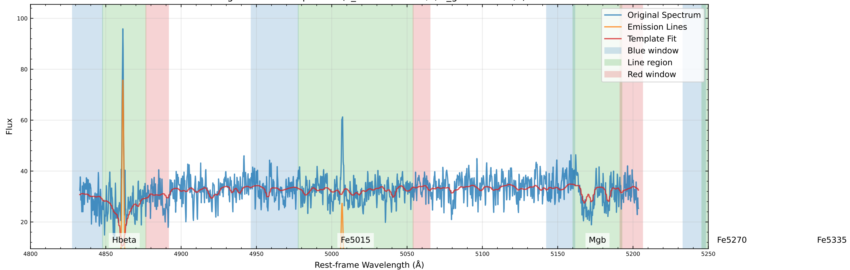
Original Data Comparison ( v_{\text{star}}=-33.7 km/s, v_{\text{gas}}=-3.1 km/s)
