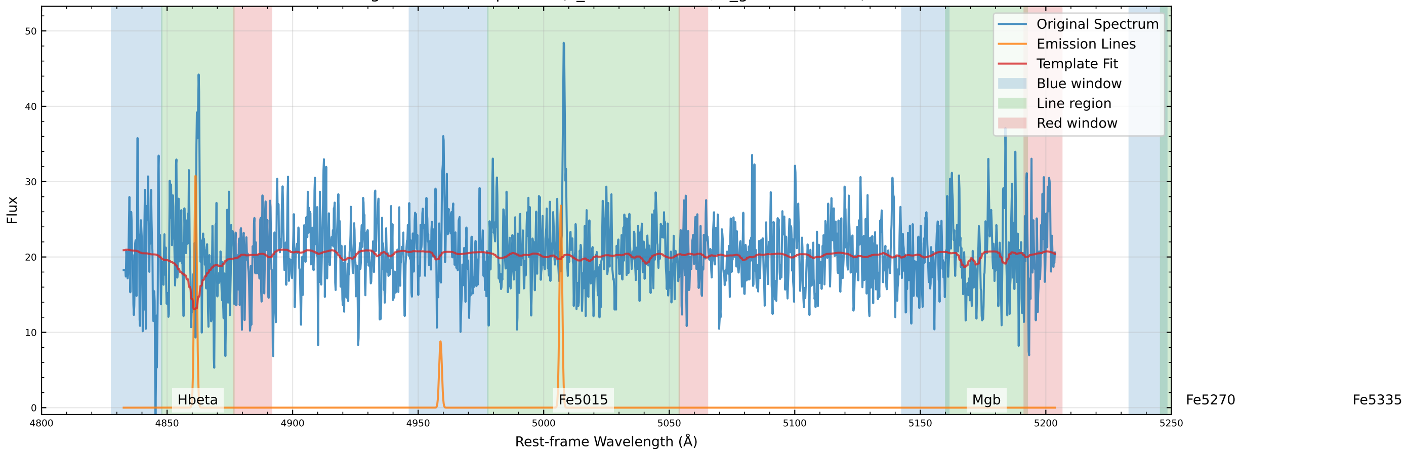
Original Data Comparison (v_star=90.5 km/s, v_gas=69.3 km/s)
